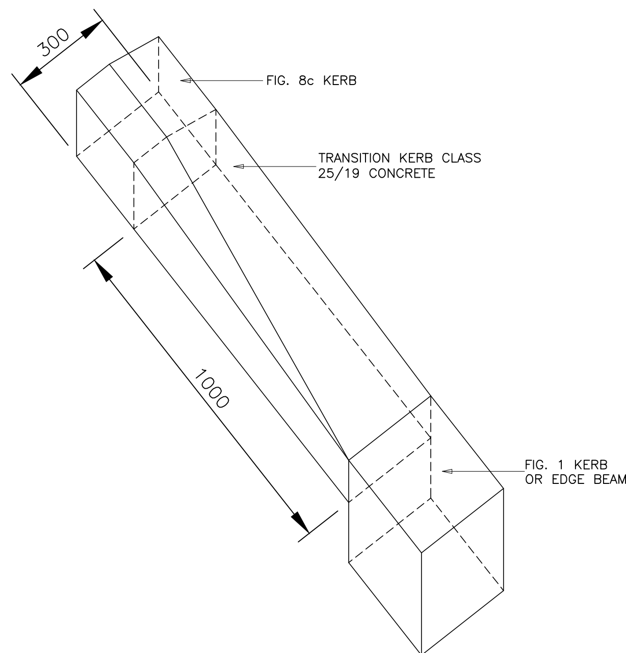
TRANSITION KERB SCALE 1:5
