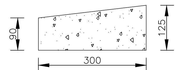
CAST IN-SITU CHANNEL (FIGURE 14) SCALE 1:2.5
