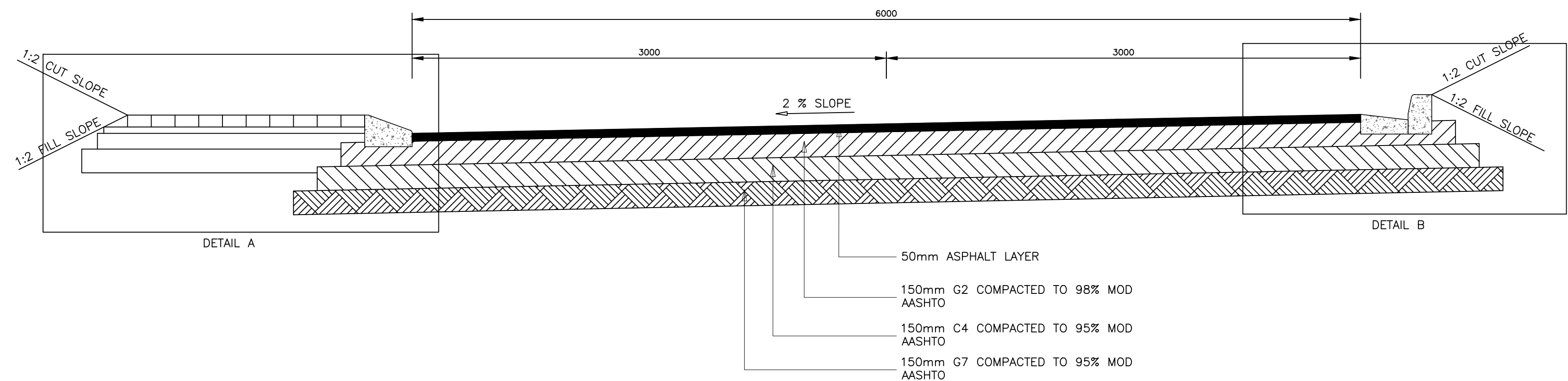
TYPICAL ROAD SECTION - 6.0m SCALE 1:10
