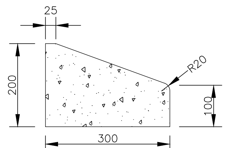
KERB - FIGURE 8c SCALE 1:2.5
