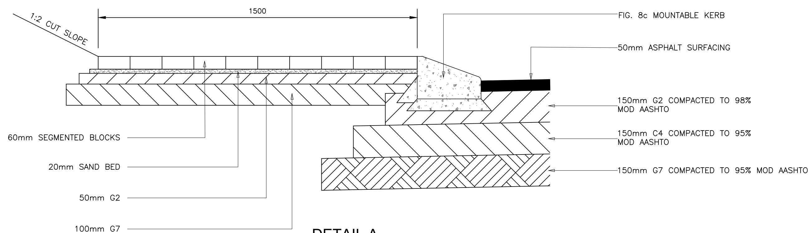
DETAIL A SCALE 1:5
