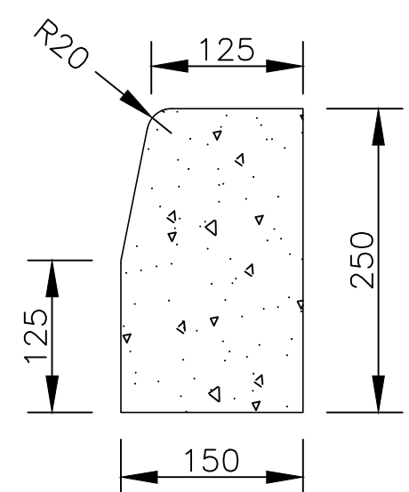
KERB - FIGURE 4 SCALE 1:2.5
