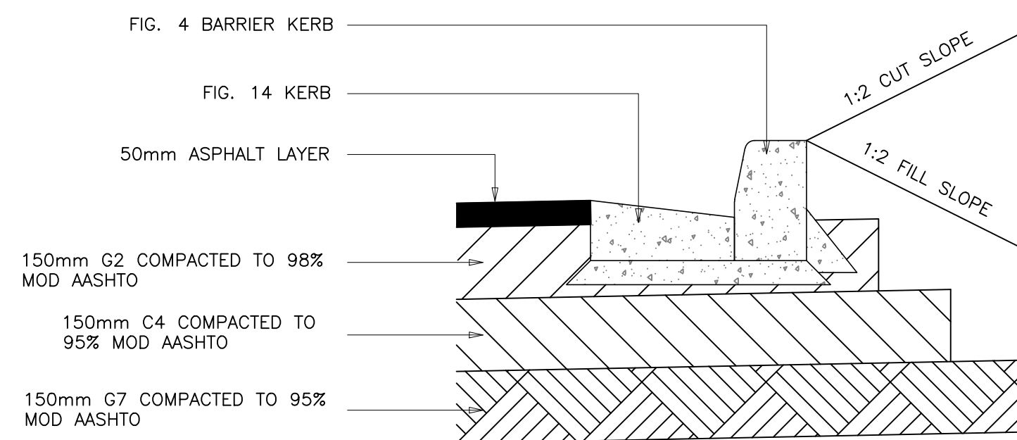
DETAIL B SCALE 1:5
